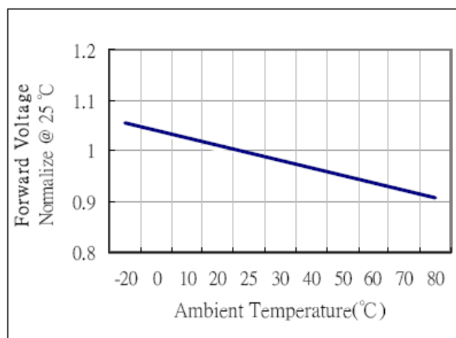
Forward voltage vs. Temperature
