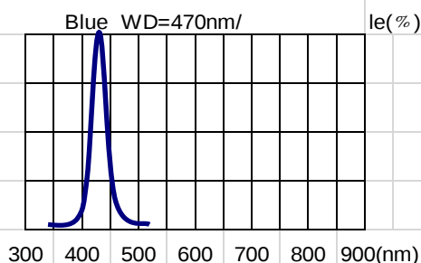
Fig.4 RELATIVE LUMINOUS INTENSITY VS. WAVELENGTH.
